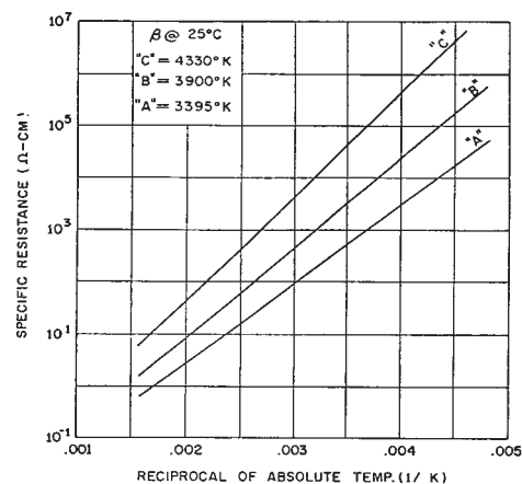
Figure 7: R-T Characteristics
