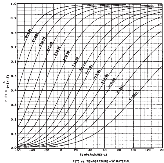
Figure 15: Design curves for “A” Material System (MIL-PRF-23648D).
