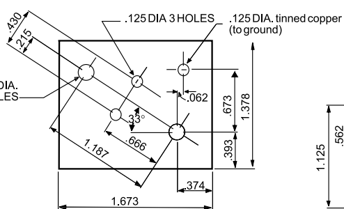
P/N 09SPS01-001 (TO-3)
