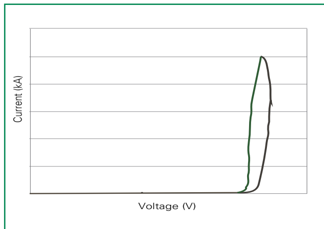
Figure 2 - Surge Response
