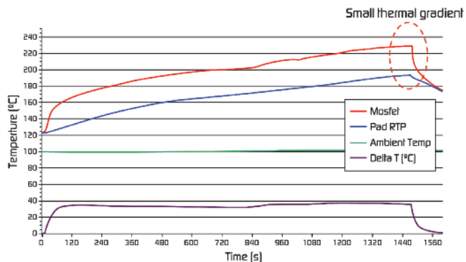
Figure 9. RTP device performance on IMS structure.
