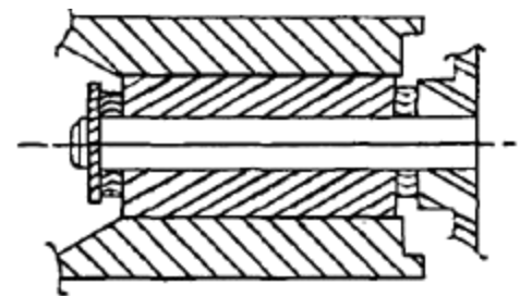
Figure 1-A Sleeve Bearing Assembly
