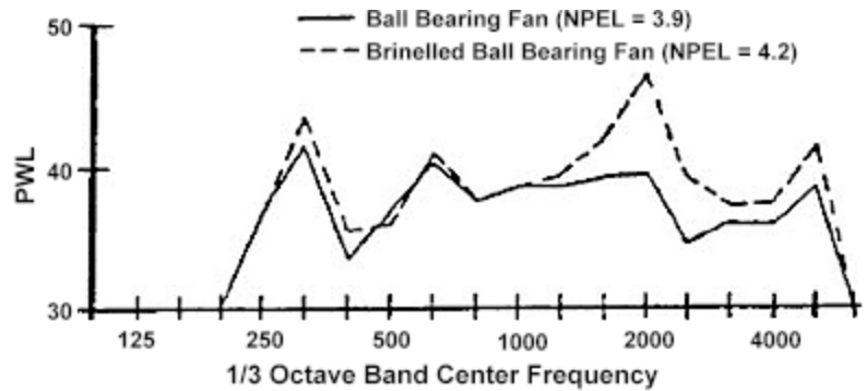
Figure 3: Fan Noise Due to Damaged Ball Bearing
