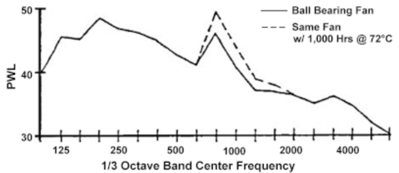
Figure 4: Fan Noise vs Life
