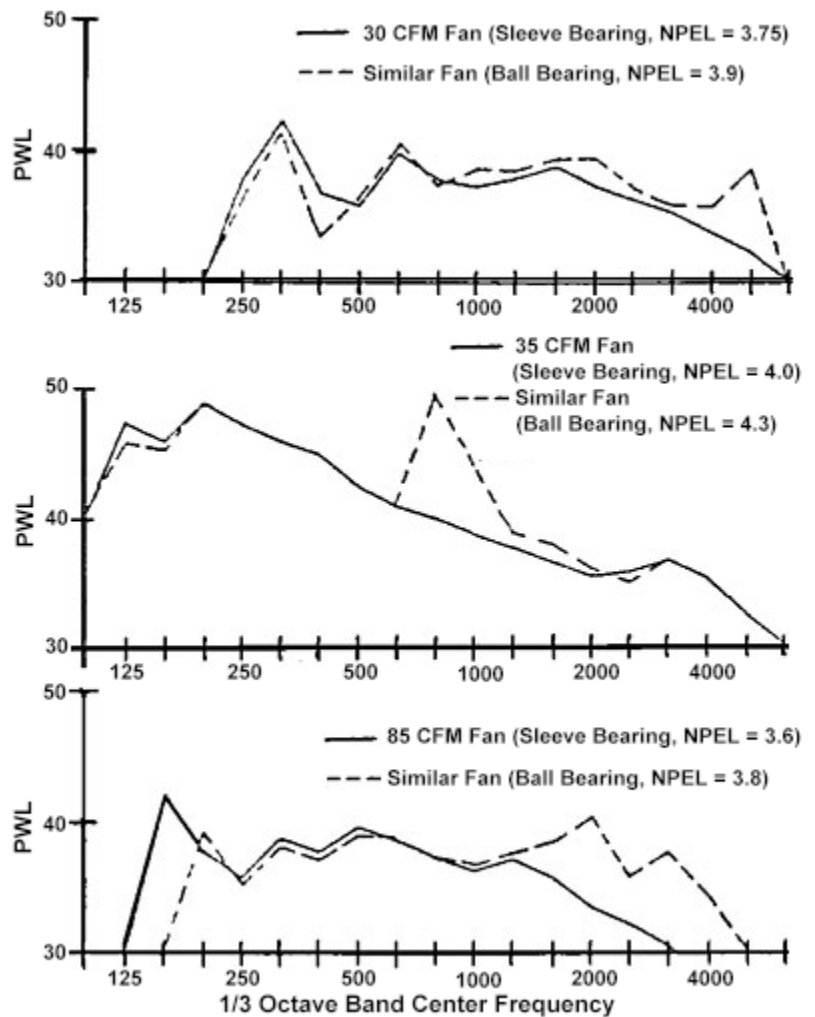
Figure 2: Sleeve Bearing vs Ball Bearing Fan Noise
