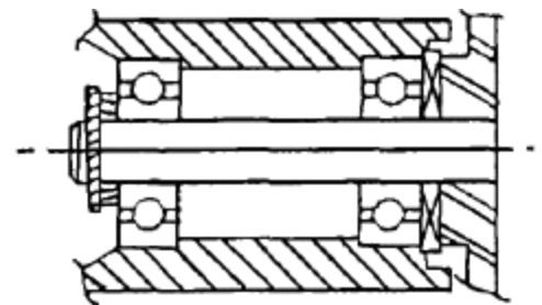
Figure 1-B Ball Bearing Assembly
