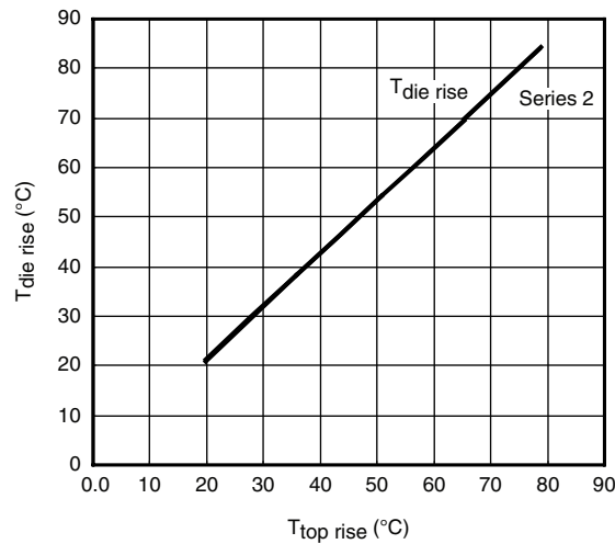
Figure 4 - Top Temperature Rise vs. Die Temperature Rise of Si4686DY
