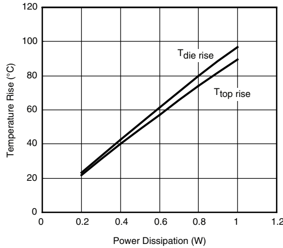
Figure 2 - Si4800BDY Top and die Temperature Rise
