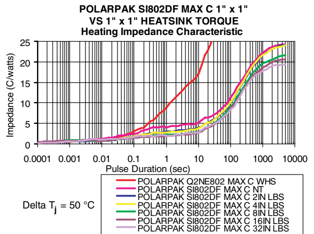
Figure 10. Transient thermal characteristics at different torque values
