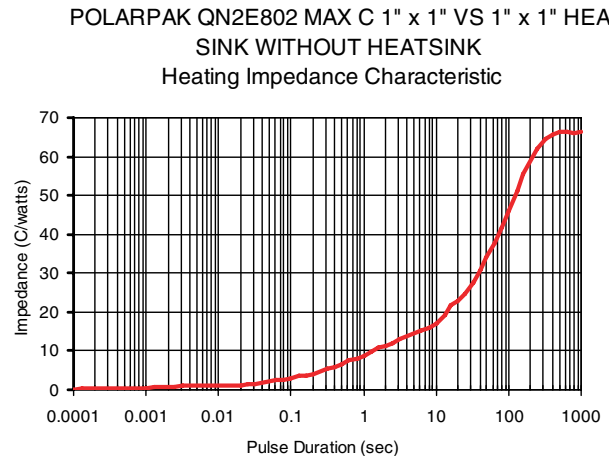
Figure 8. Transient thermal impedance characteristics
