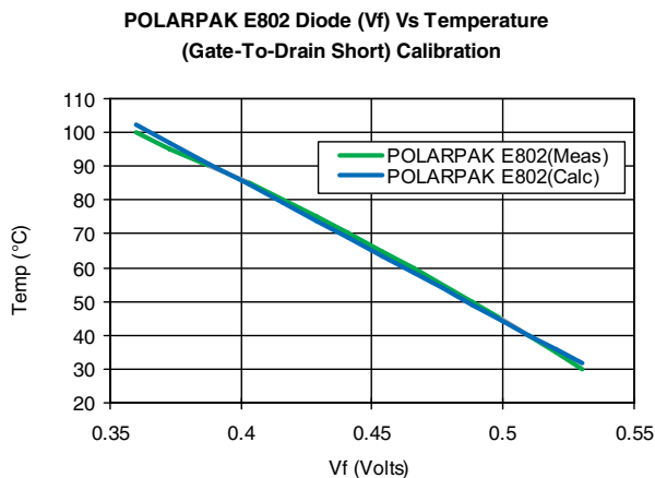
Figure 6. Calibration
