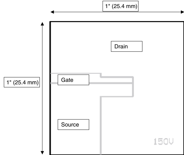
Figure 1. PC board design
