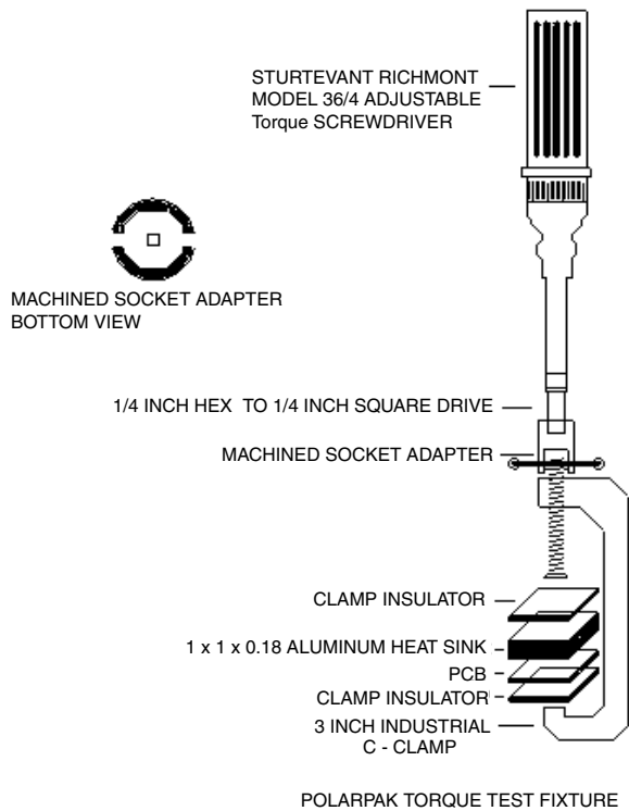
Figure 9a. Complete clamping and torque setting arrangement
