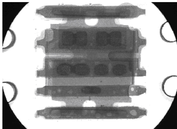
Figure 11b. X-Ray of damaged part
