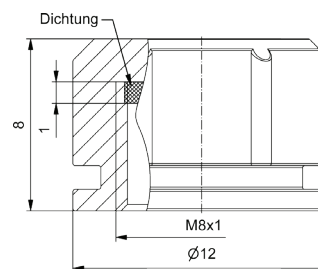
Dimension Male connector
