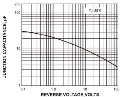
FIG. 5-TYPICAL JUNCTION CAPACITANCE
