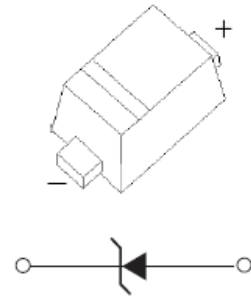
SOD-523
