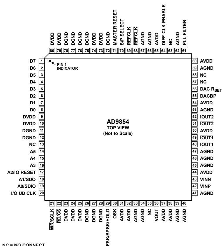
Figure 2. Pin Configuration
