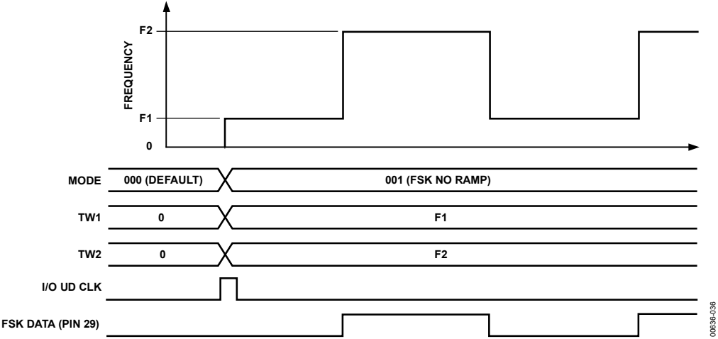
Figure 36. Unramped (Traditional) FSK Mode
