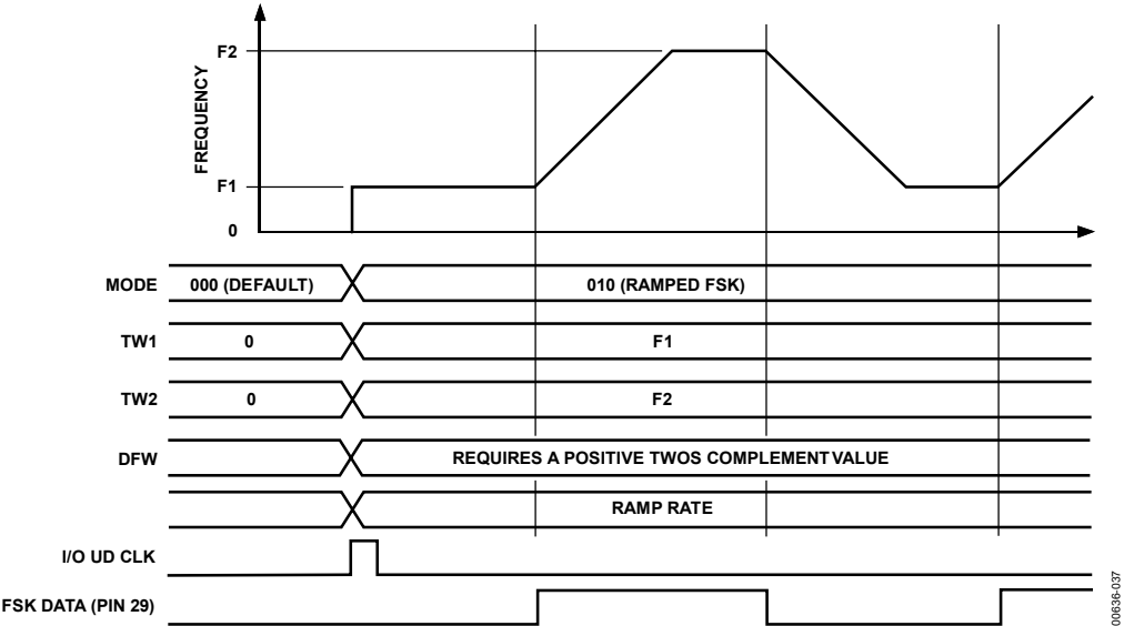
Figure 37. Ramped FSK Mode (Start at F1)
