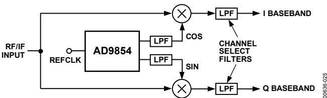
Figure 25. Quadrature Downconversion
