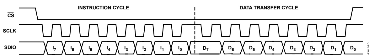
Figure 60. Serial Port Write Timing Clock Stall High
