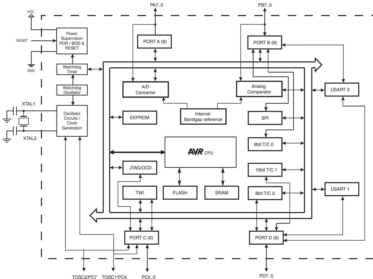
Figure 2-1. Block Diagram
