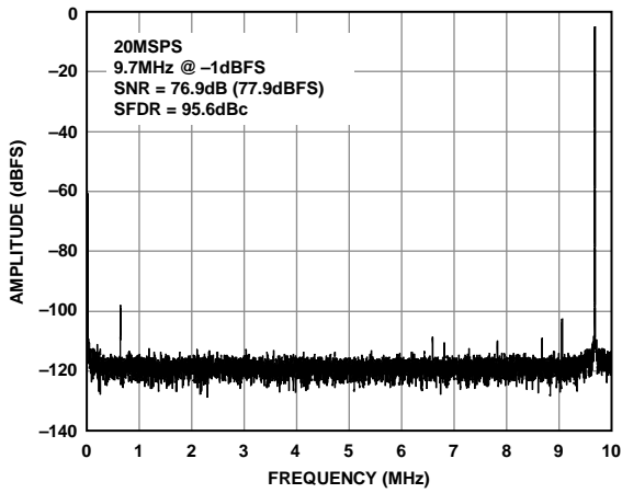
Figure 24. AD9266-20 Single-Tone FFT with f_{IN} = 9.7 MHz
