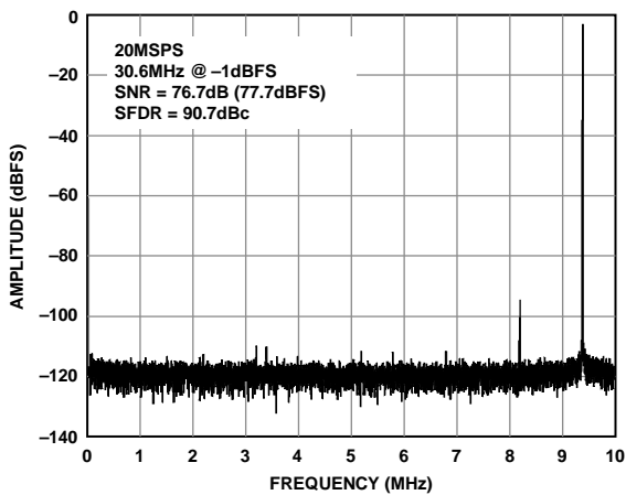
Figure 25. AD9266-20 Single-Tone FFT with f_{IN} = 30.6 MHz
