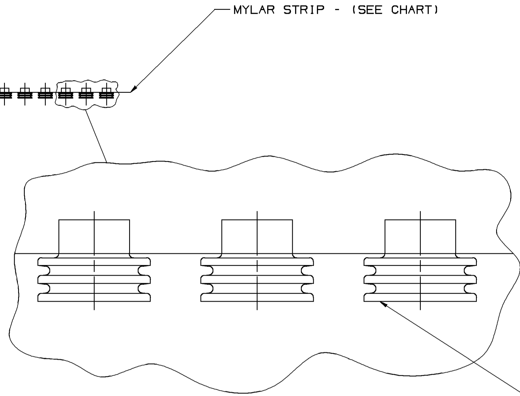
SEAL/MYLAR ASSEMBLY DETAIL
