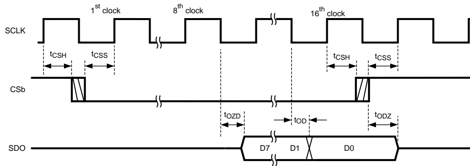
Figure 54. Read Timing
