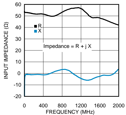
Figure 38. Input Impedance
