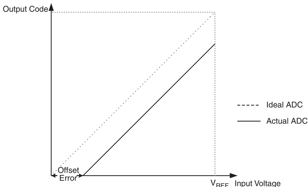
Figure 13-9. Offset Error
