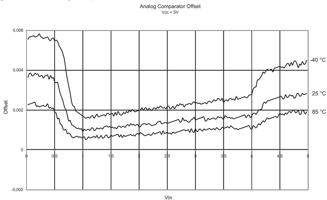
Figure 17-36. Analog Comparator Offset
