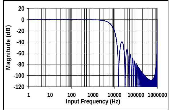
图 B-3: SINC 滤波器响应 (MCLK = 4 MHz, OSR = 64, PRESCALE = 1)
