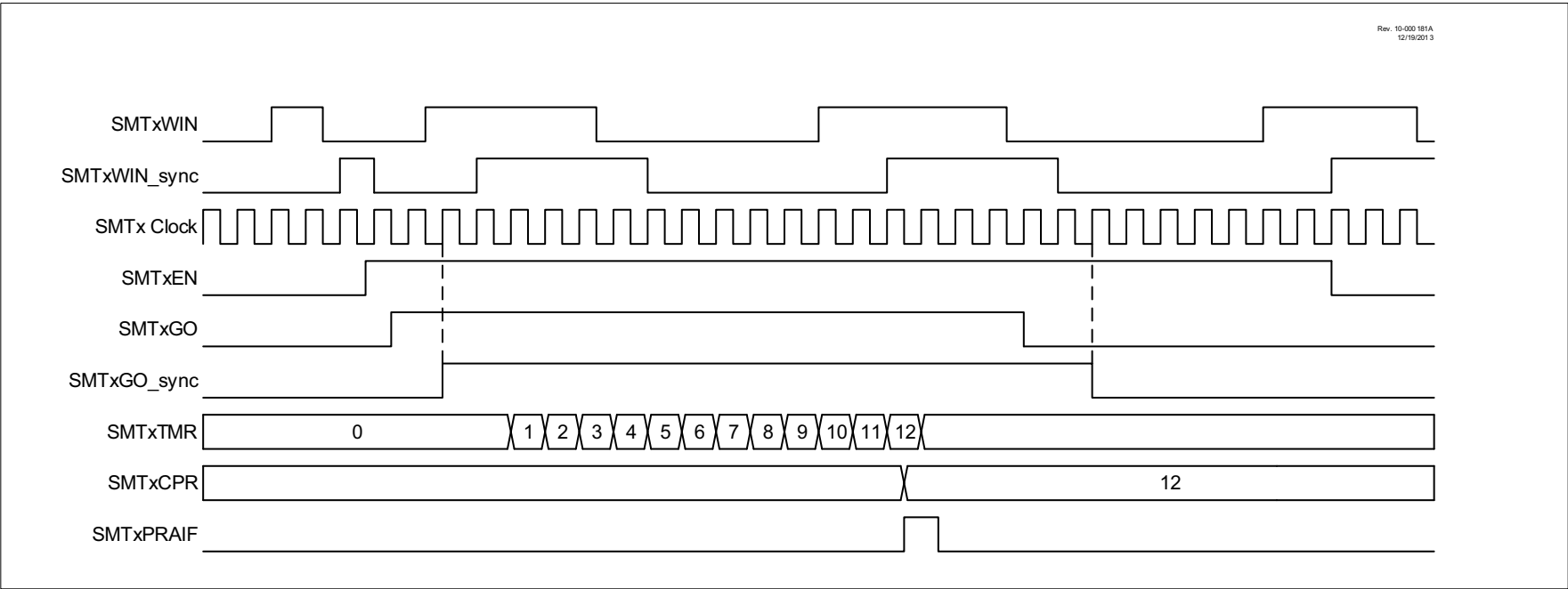
FIGURE 32-11: WINDOWED MEASURE MODE SINGLE ACQUISITION TIMING DIAGRAM
