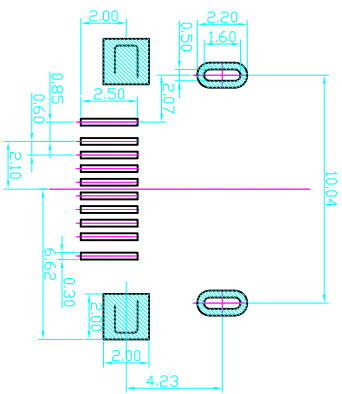
RECOMMENDED PCB LAYOUT TYPE VIEW GENERAL TOLERANCE +/- 0.05
