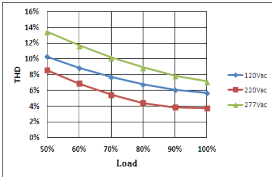
THD Curve(Ref.)
