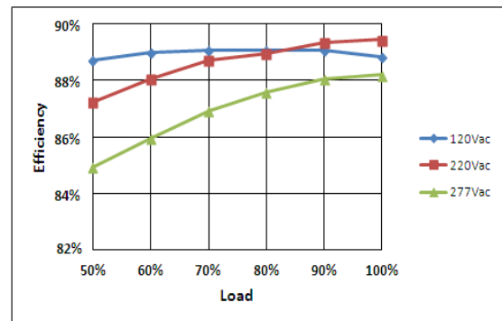
Efficiency VS. Load Curve(Ref.)
