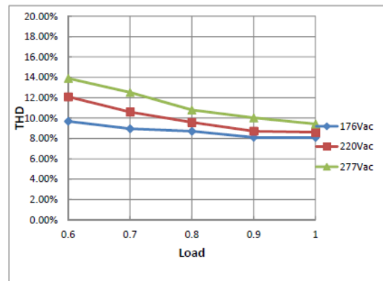
THD Curve
