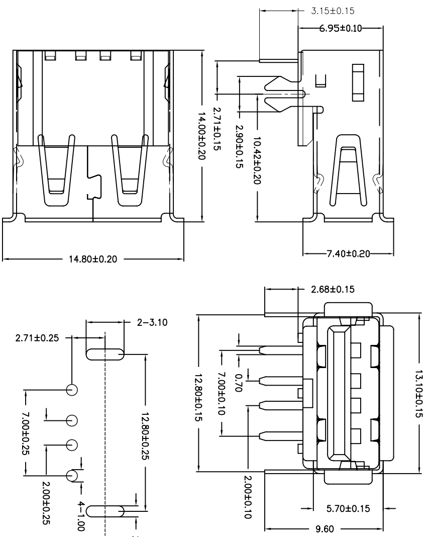
PCB LAYOUT
