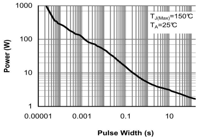
Figure 10: Single Pulse Power Rating Junc to-Ambient (Note E)
