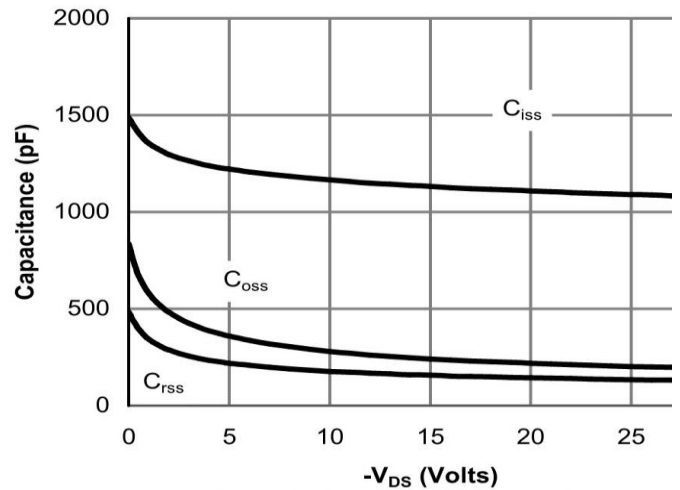
Figure 8: Capacitance Characteristics
