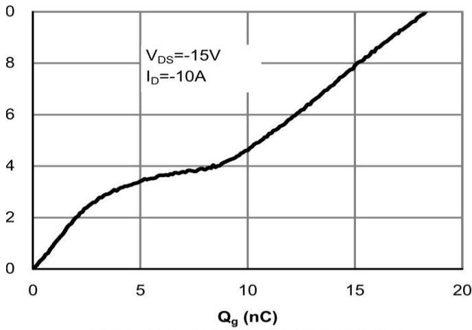
Figure 7: Gate-Charge Characteristics
