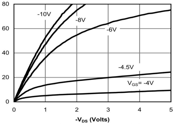
Figure 1: On-Region Characteristics
