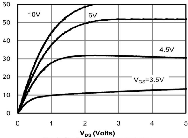
Fig 1: On-Region Characteristics
