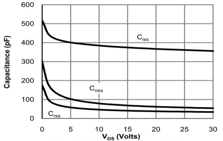
Figure 8: Capacitance Characteristics
