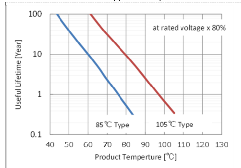
Useful Lifetime for Mobile Application Specific MLCC
