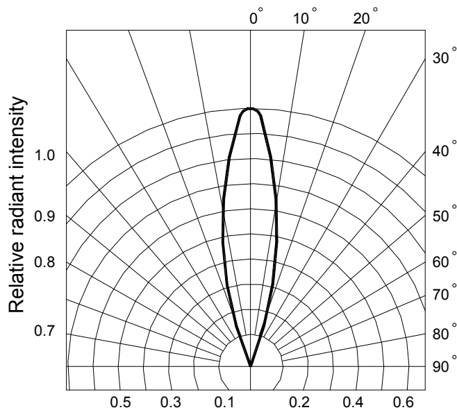
Fig.6 Radiation diagram
