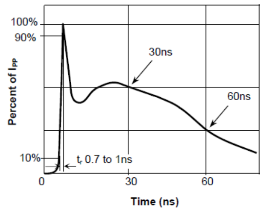
Fig.4 Pulse Waveform-ESD(IEC61000-4-2)
