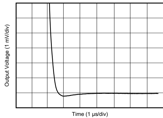
G = 1 C_L = 100\text{ pF} 2\text{-V step} D031
