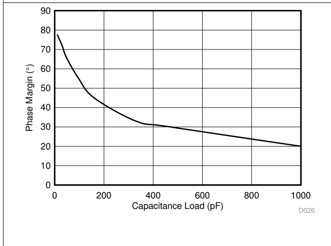
Figure 20. Phase Margin vs Capacitive Load
