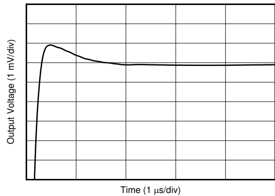
G = 1 C_L = 100\text{ pF} 2\text{-V step} D032
