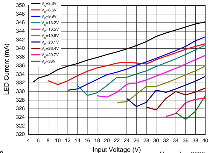
LED Current vs. Input Voltage (TSOT25, R_S=0.3\Omega , L=100\mu\text{H} )
