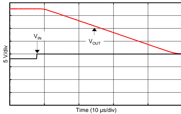
Figure 23. Positive Overload Recovery
