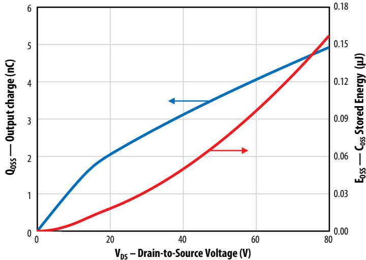
Figure 5c: Output Charge and C_{OSS} Stored Energy
