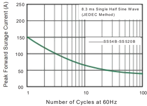
Fig .5 Maximum Non- Repetitive Peak Forward Surge Current
