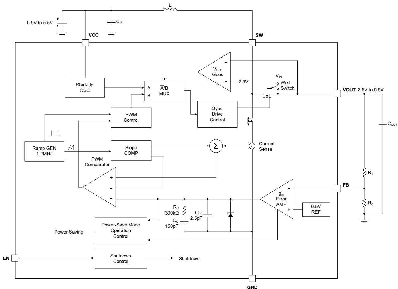
Figure 4. Block Diagram
