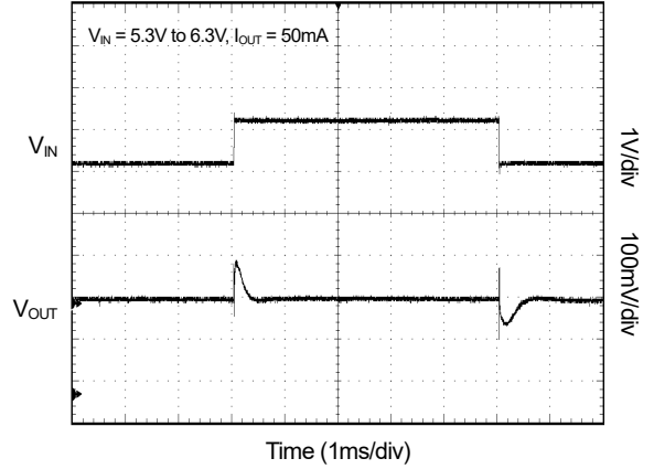
Line-Transient Response
