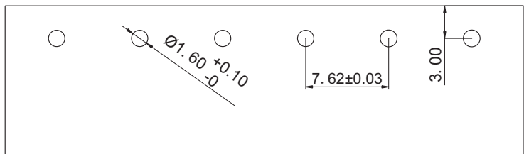
PCB Layout
