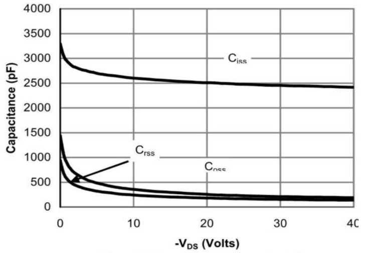
Figure 8: Capacitance Characteristics
