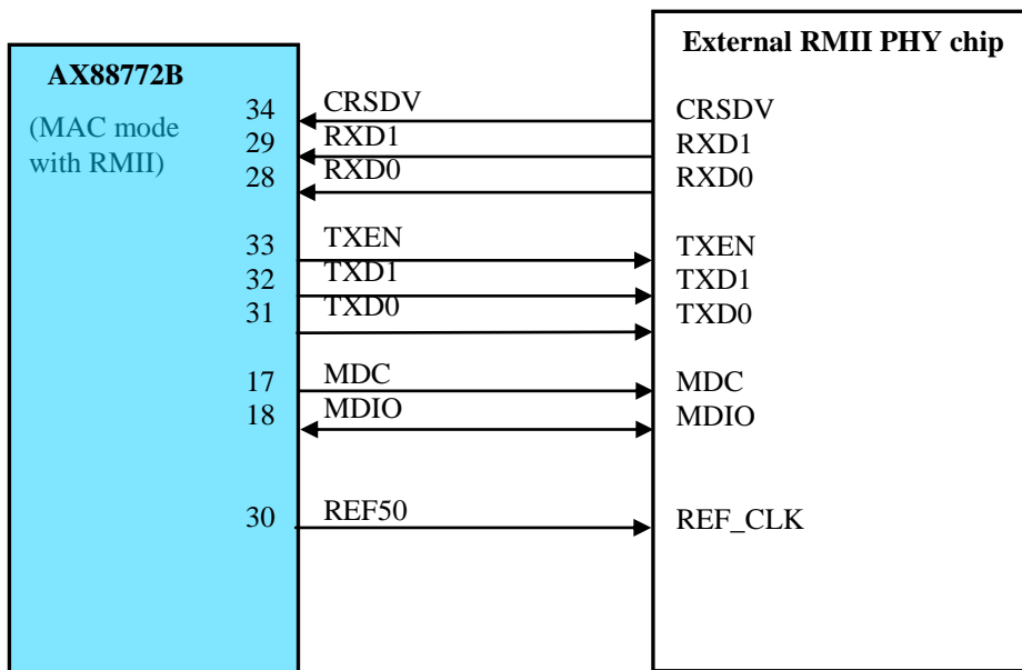
Figure 10 : RMI2 Interface to External PHY chip
