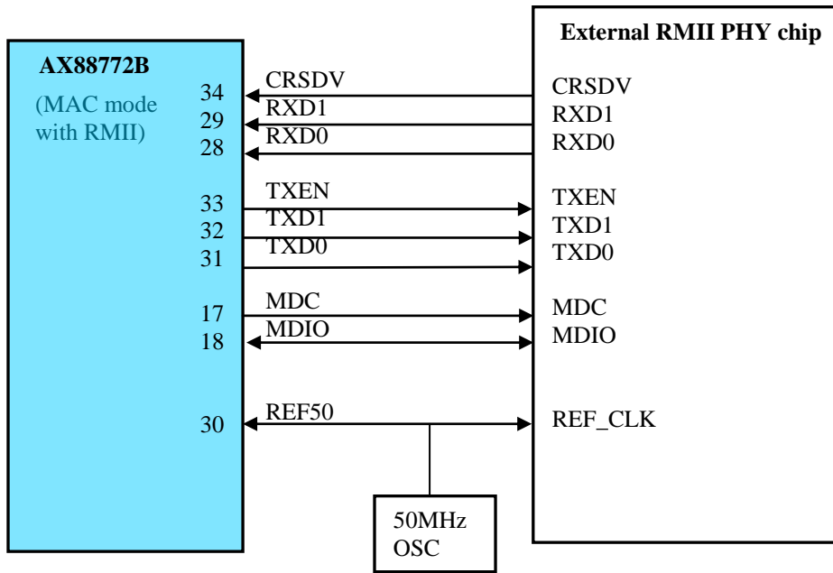
Figure 9 : RMI2 to External PHY chip with 50MHz OSC
