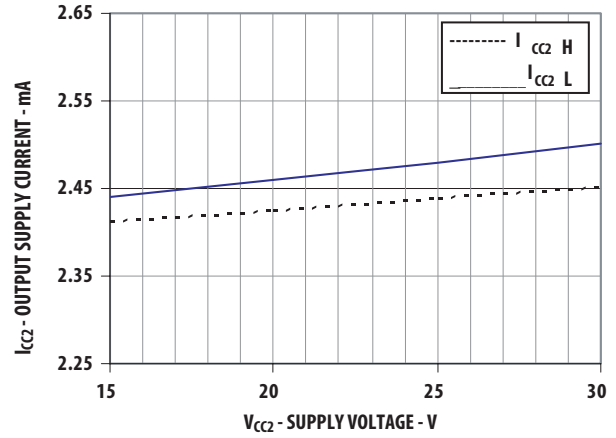
Figure 7. I_{C2} vs. V_{C2}
