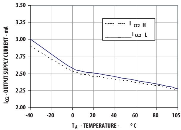
Figure 6. I_{C2} vs. temperature
