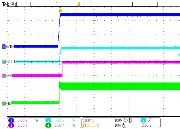
Figure 10. Power up
