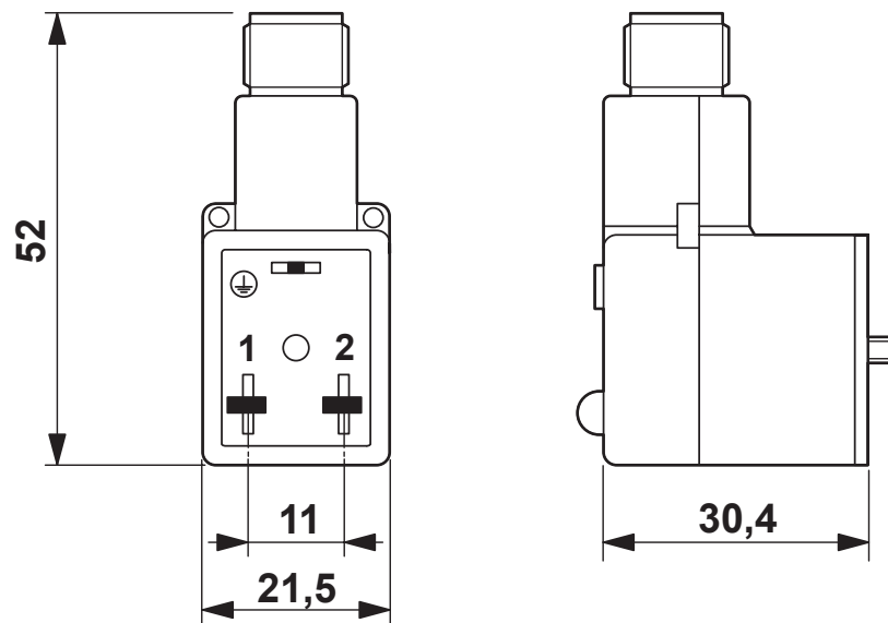
Dimensional drawing
