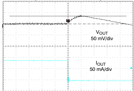
Figure 22. 100 mA to 10 mA Load Transient ( V_{IN} = 3.6\text{ V} , V_{OUT} = 1.2\text{ V} , T_A = 25^\circ\text{C} )
