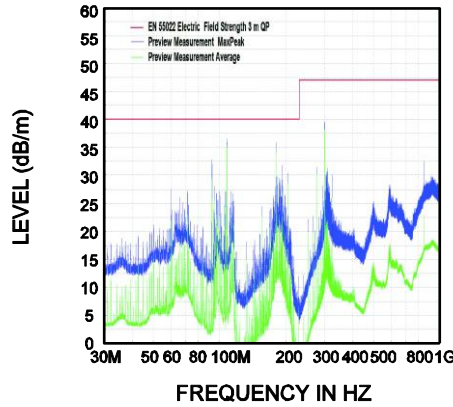
Radiated EMI
