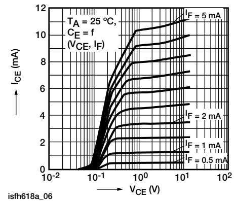
Fig. 8 - Output Characteristics
