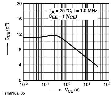
Fig. 7 - Transistor Capacitance
