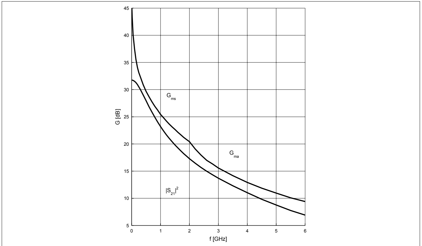
Figure 8 Gain G_{ma}, G_{ms}, IS_{21}^2 = f(f), V_{CE} = 3 \text{ V}, I_C = 25 \text{ mA}
