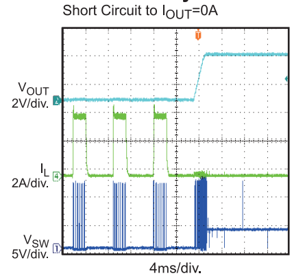
SCP Recovery Short Circuit to I_{OUT} = 0A
