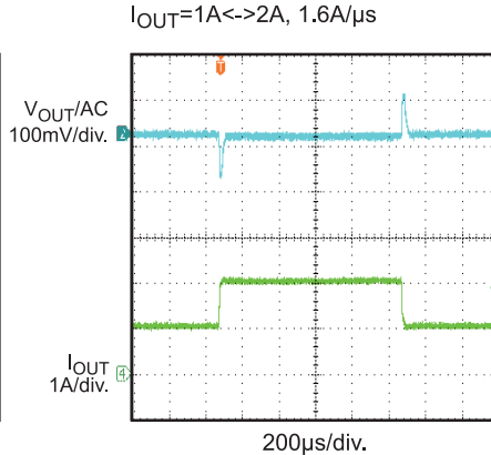
Load Transient I_{OUT} = 1A \leftrightarrow 2A, 1.6A/\mu s
