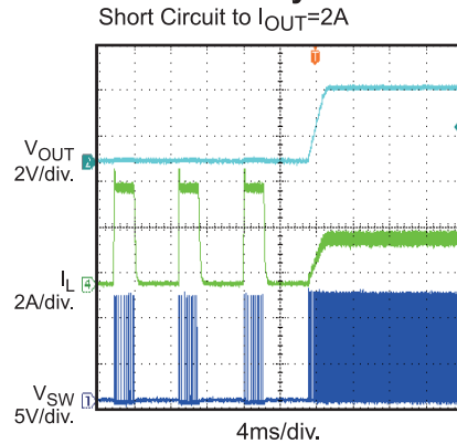
SCP Recovery Short Circuit to I_{OUT} = 2A
