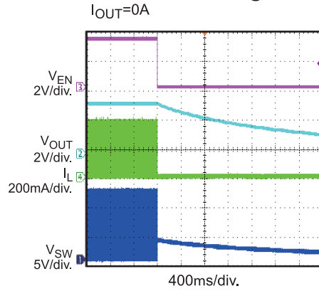
Shutdown Through EN I_{OUT} = 0A
