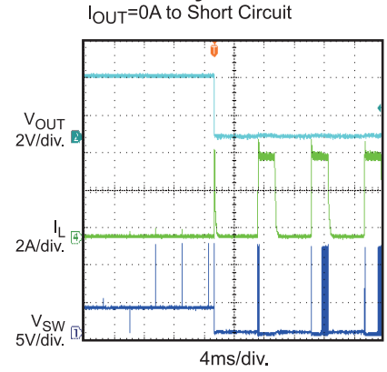
SCP Entry I_{OUT} = 0A to Short Circuit
