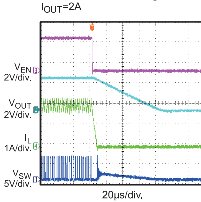
Shutdown Through EN I_{OUT} = 2A
