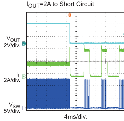
SCP Entry I_{OUT} = 2A to Short Circuit
