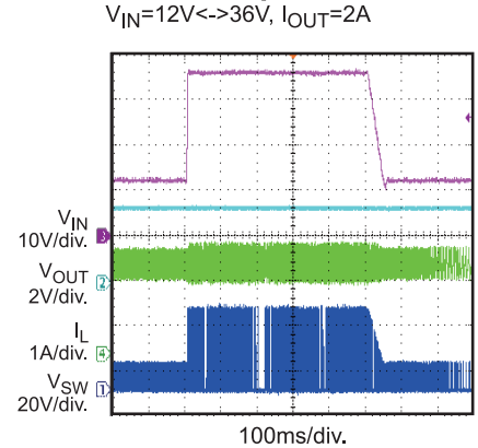
Load Dump V_{IN} = 12V \leftrightarrow 36V, I_{OUT} = 2A
