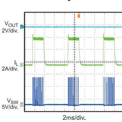
SCP Steady State
