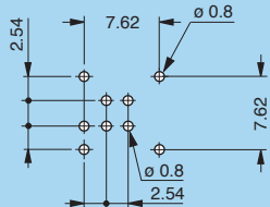
P19 - EPG-EXG (0B/1B.305) Solder mount
