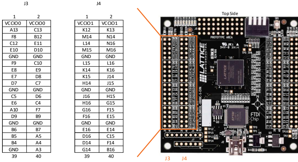
Figure 7.1. J3/J4 Header Landing Callout
