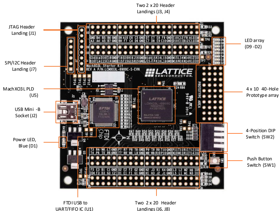
Figure 2.1. MachXO3 Board (MachXO3L Version), Top Side
