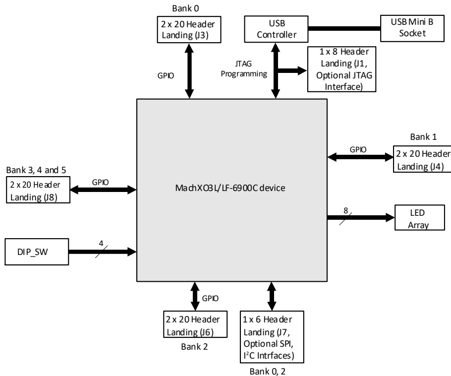
Figure 6.1. MachXO2 and MachXO3L/LF-6900C Block Diagram
