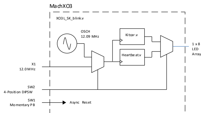
Figure 6.2. Demonstration Design Block Diagram
