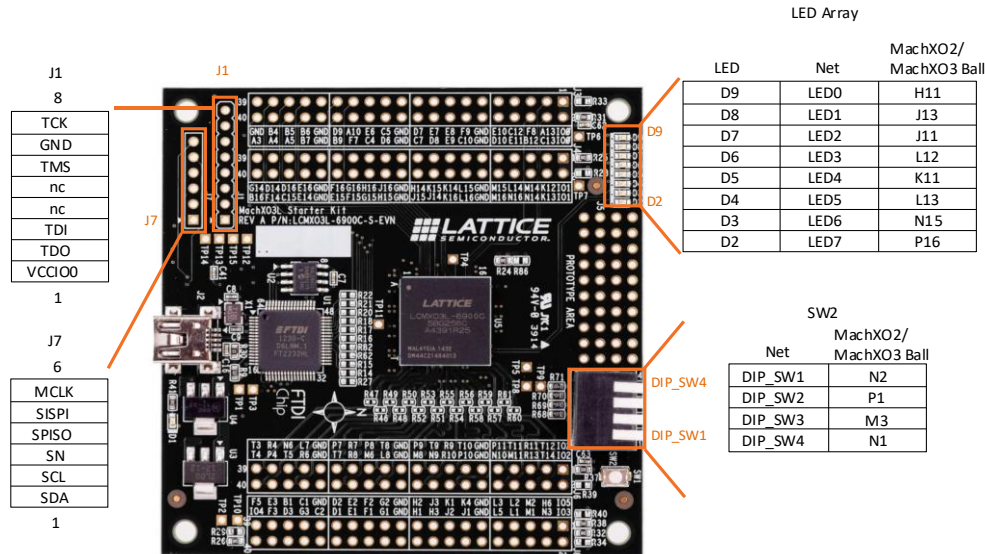
Figure 7.3. J1 Header Landing and LED Array Callout
