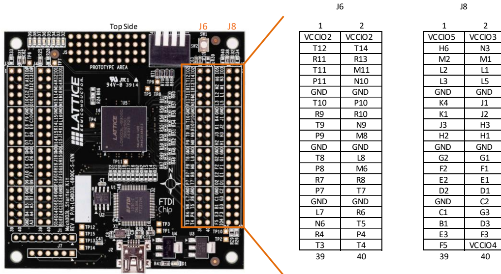
Figure 7.2. J6/J8 Header Landing Callout
