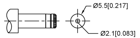
MATING PLUG Jack Insertion Depth: 9.15 mm
