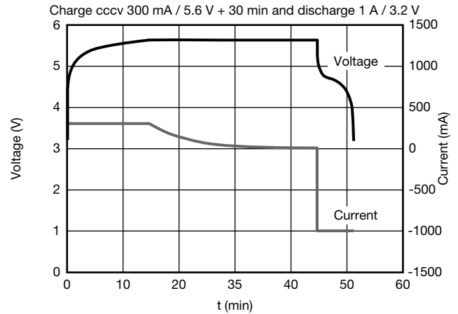
Fig. 26 - Constant Current (CC)-Constant Voltage (CV) Charging Method at RT Typical Charge / Discharge Characteristics at RT: 90 F / 5.6 V
