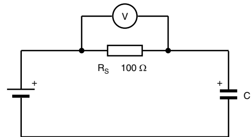
Fig. 16 - Test Circuit for Leakage Current
